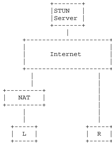
Figure 7: Example Topology
